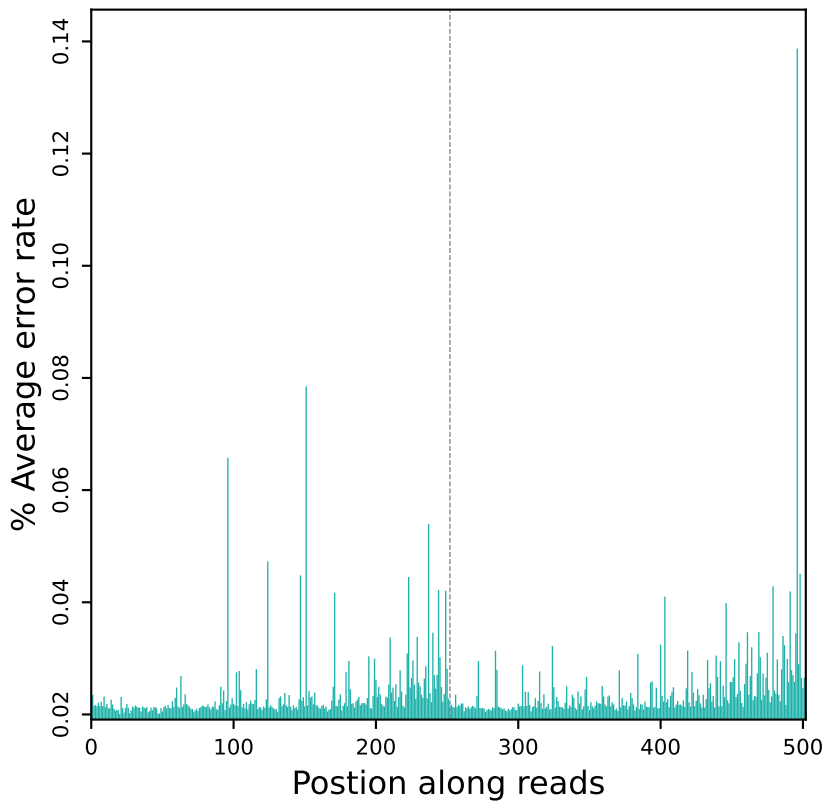
Error rate distribution along reads (R10905)
